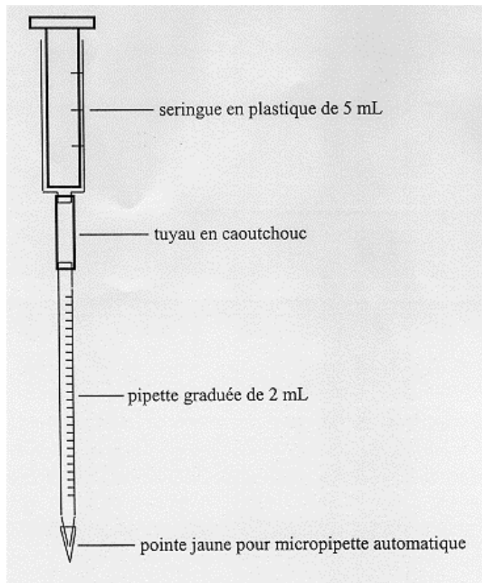
Figure 3 : Microburette.
